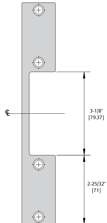
1N-2 Faceplate Option
